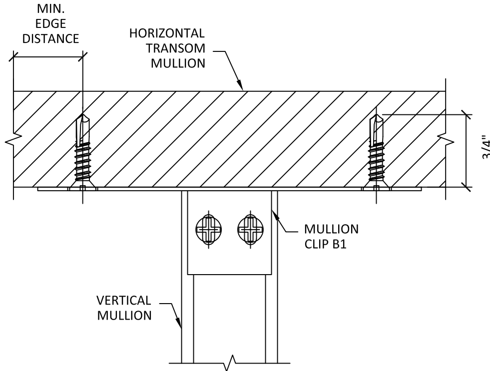
B 3 INSTALLATION DETAIL CLIP B1 INSTALLATION
